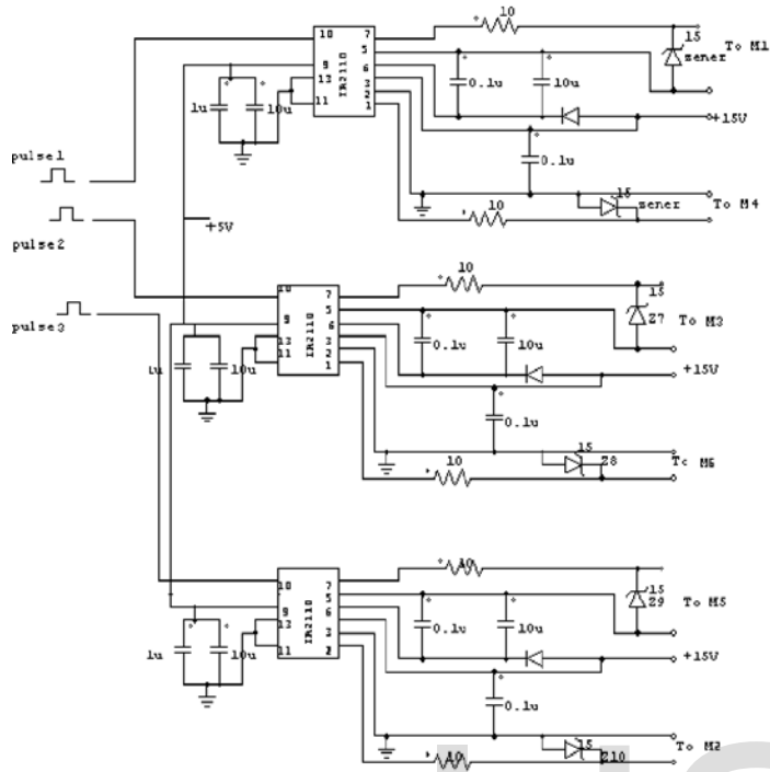
Fig 1.3 Driver Circuit
