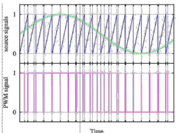
Fig 1.2 PIC output waveform
